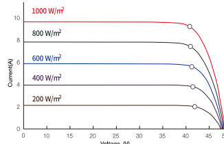
I-V curve
