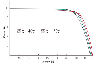
I-V curve
